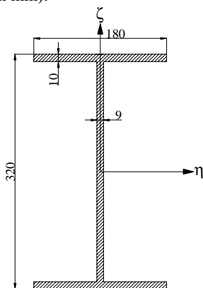
Fig. 2 Cross-section scheme
