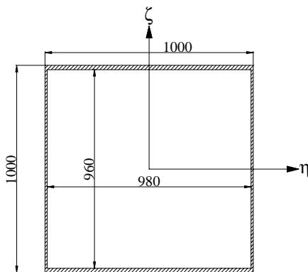
Fig. 9 Cross-section scheme
