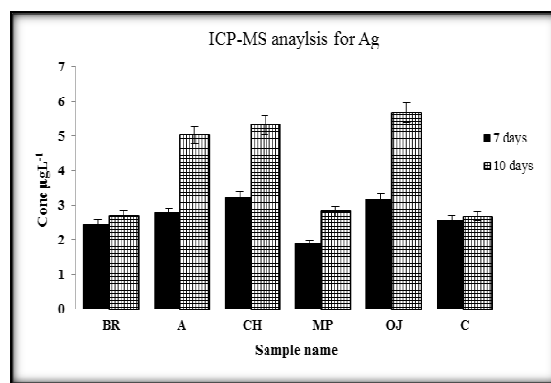
Fig. 7 ICP-MS determination of Ag migration from antimicrobial containers into specified foodstuffs for 7 and 10 days at 40^\circ\text{C}
