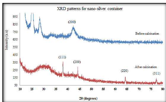
Fig. 5 XRD patterns for Ag and \text{TiO}_2 nanoparticles in antimicrobial container polymer
