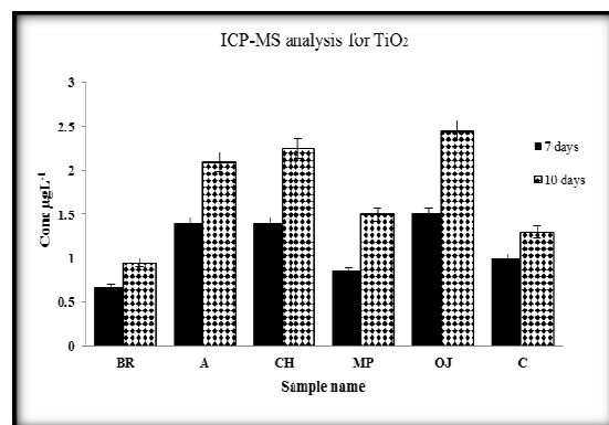
Fig. 8 ICP-MS determination of Ti migration from antimicrobial containers into specified foodstuffs for 7 and 10 days at 40^\circ\text{C}
