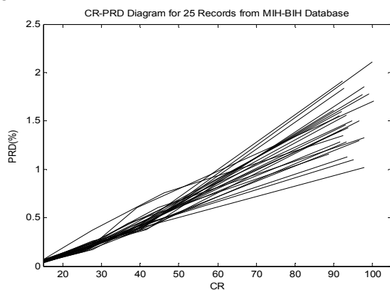
Fig. 4 CR-PRD results for 25 records from MIT-BIH database
