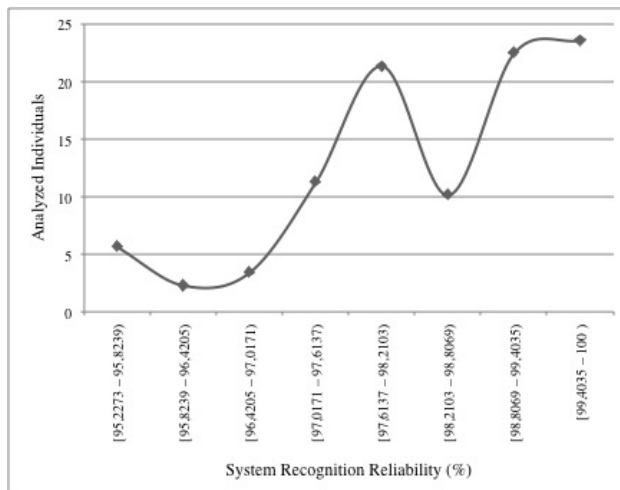
Fig. 15 Features Reliability
