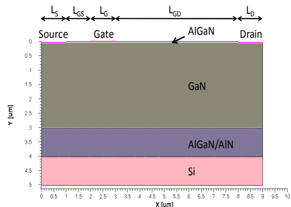
Fig. 1 The cross-section view of AlGa N /Ga N HEMT device model structure
