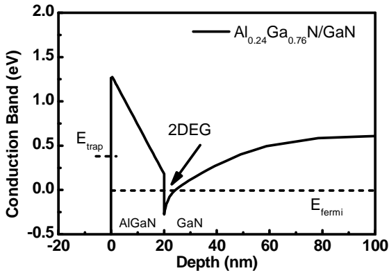
Fig. 2 The conduction band diagram of AlGaIn/GaN hetero-junction
