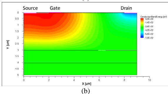
Fig. 15 The conduction band distribution profile of (a) standard AlGaIn/GaN HEMT at V_{GS} = -5.5 V and V_{DS} = 268 V (b) AlGaIn/GaN HEMT with GaN cap and AlN spacer at V_{GS} = -5.5 V and V_{DS} = 630 V
