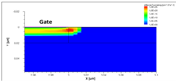
Fig. 9 The zoom-in gate electron tunneling distribution profile of AlGaIn/GaN HEMT at V_{GS} = -6 V and V_{DS} = 10 V
