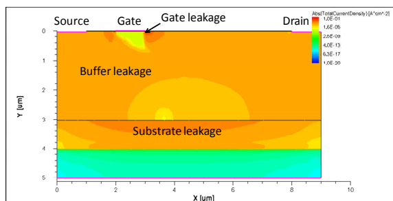
Fig. 7 The current density distribution profile of AlGaIn/GaN HEMT at V_{GS} = -6 V and V_{DS} = 10 V
