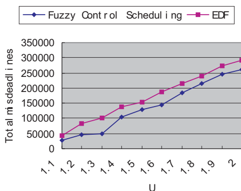
Fig. 4: Total misdeadlines
