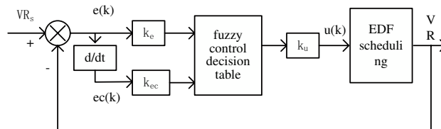
Fig. 1: Fuzzy control scheduling
