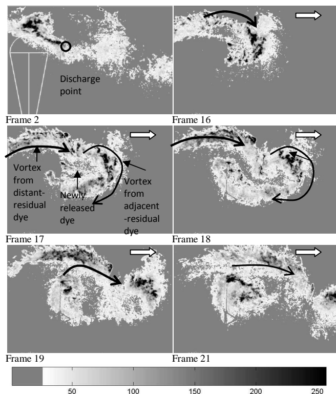
Fig. 6 PLIF images of dye concentration distribution for dye discharge at point B2, tidal flow, ( KC = 6.9 , T = 60s ). All curved arrows indicate movement of residual dye. White arrows on top right corner indicate eastward or westward ambient flow
