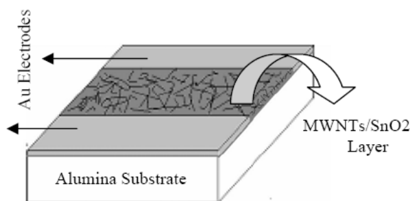
Fig. 1 Schematic diagram of MWNTs/ SnO 2 sensor lay-out
