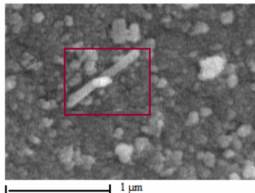
Fig. 2: SEM images of nanocomposite MWNTs/SnO 2 .
