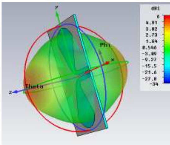
Fig. 5 3D radiation pattern at 8 GHz
