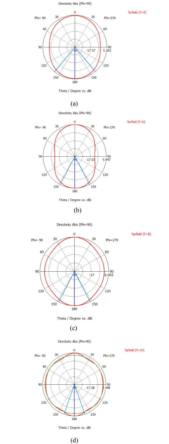
Fig. 4 Simulated radiation patterns in the H-plane at (a) 4GHZ (b) 6 GHz (c) 8 GHZ and (d) 10 GHZ
