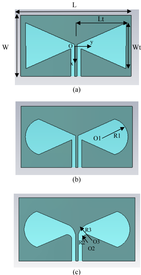
Fig. 1 Antennas geometry (a) triangular bowtie (b) with rounded ends (c) with rounded ends and progressive feed line
