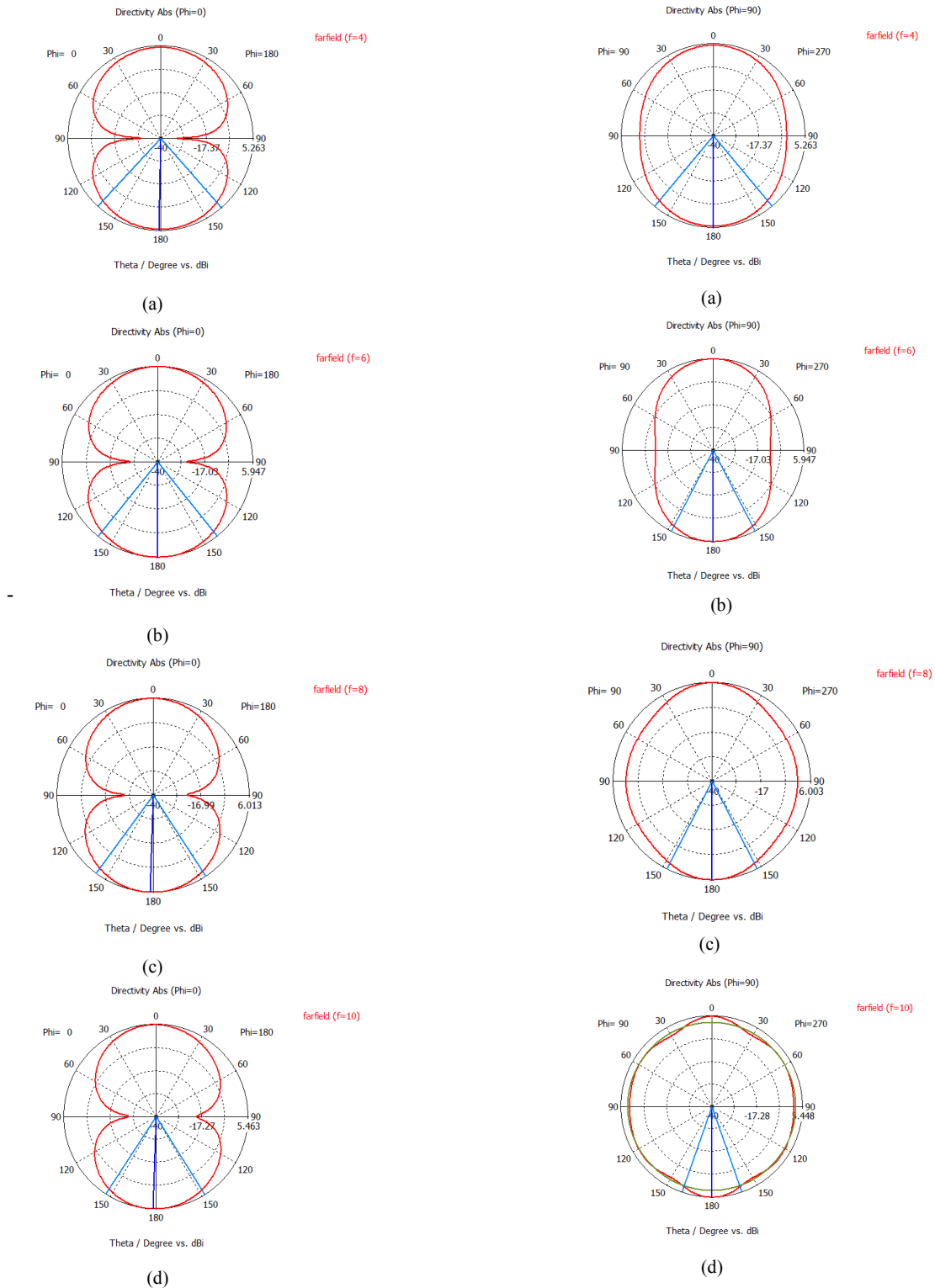
Fig. 3 Simulated radiation patterns in the E-plane at (a) 4GHZ (b) 6 GHz (c) 8 GHZ and (d) 10 GHZ
