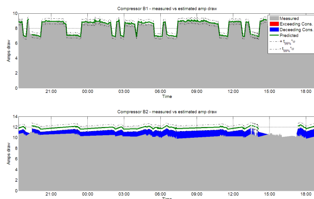
Fig. 6 Compressor amps draw monitoring
