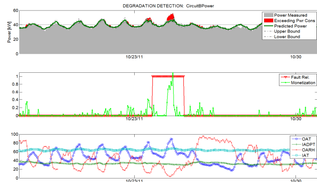
Fig. 5 Degradation detection example - worse performance than last season for certain driving condition was detected
