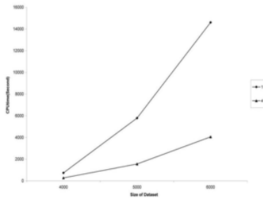
Fig. 7 Runtime over Size of Dataset
