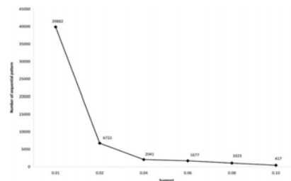
Fig. 5 number of sequences over support value
