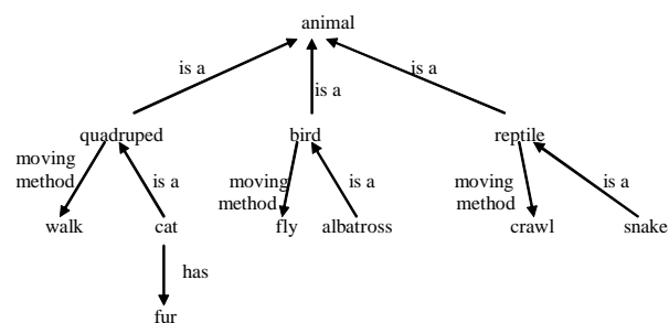
Fig. 6 A sample semantic network
