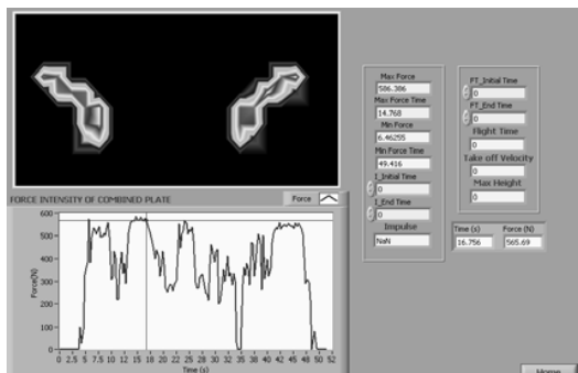
Fig. 8 Force-Logger in combine mode
