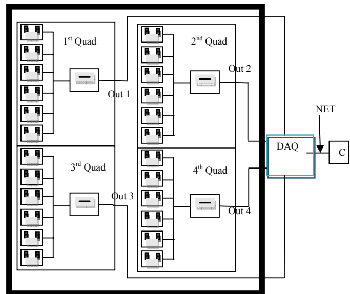
Fig. 4 Schematic diagram of arrangements of sensors into quadrants with connectivity to the ethernet
