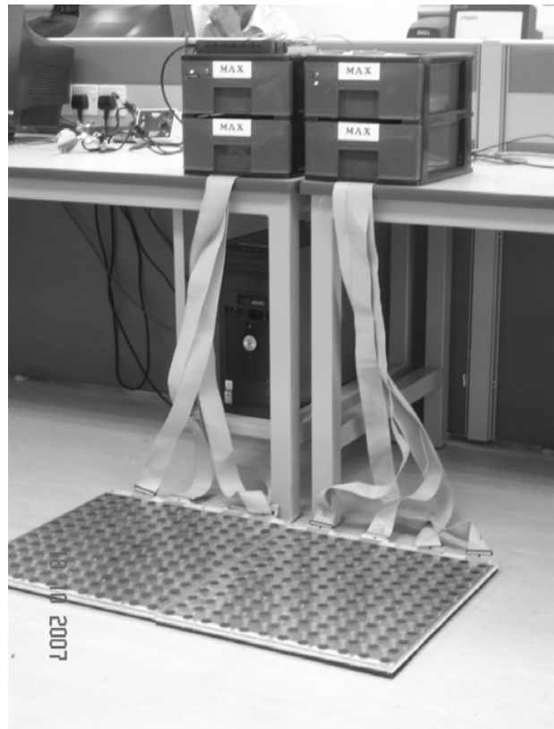
Fig. 6 Complete force platforms with four control boxes
