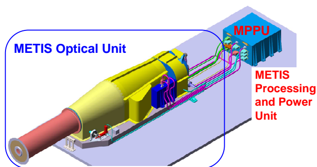
Fig. 1 METIS Coronagraph (courtesy of Thales Alenia Space Italia)
