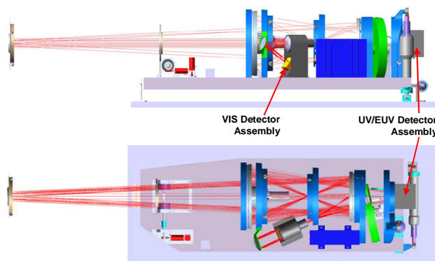
Fig. 2 METIS subsystems configuration, showing the position of the detectors assemblies (courtesy of Thales Alenia Space Italia)
