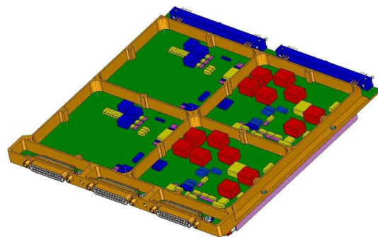
Fig. 5 MPPU electronics boards layout (courtesy of Thales Alenia Space Italia)
