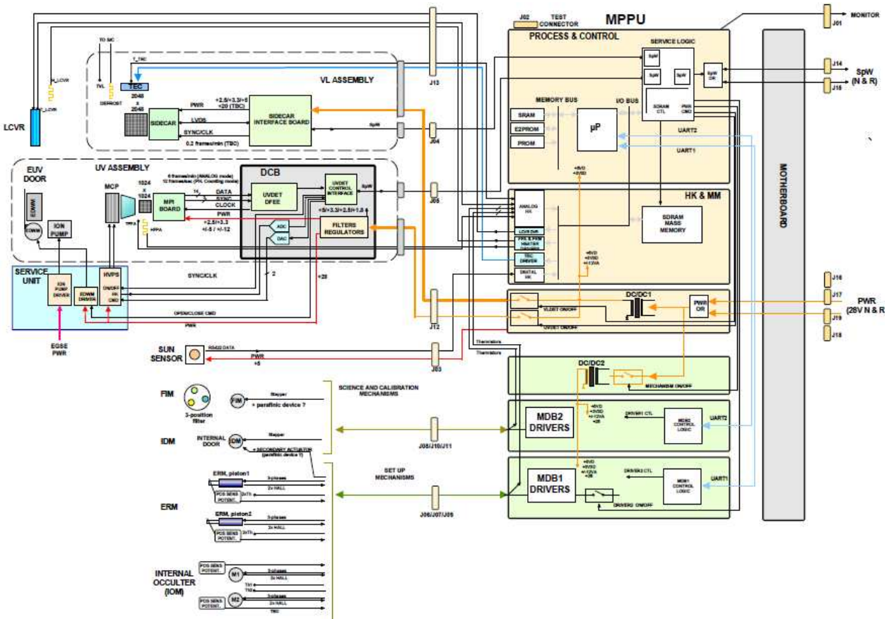
Fig. 3 METIS electronics block diagram showing the MPPU, detector assemblies and subsystems (courtesy of Thales Alenia Space Italia)
