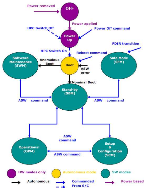
Fig. 4 METIS Operative Modes and the bootstrap procedure ending in the Stand-by mode (courtesy of Thales Alenia Space Italia)
