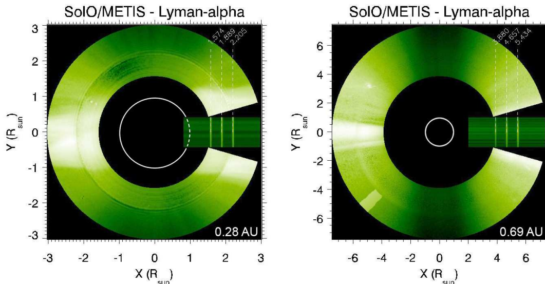
Fig. 6 METIS UV/EUV channel simulated images of the solar corona during the nominal mission's first orbit. Left: instrument's perihelion field of view @ 0.28 AU. Right: instrument's highest helio-latitude field of view @ 0.69 AU. The white circles represent the apparent diameter of the Sun, while the rectangle area on the right sides is the spectra produced by slits and diffraction grating
