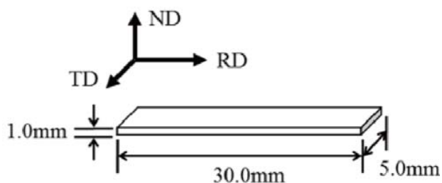
Fig. 1 Dimensions and directions of bending specimen
