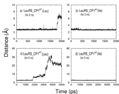
Fig. 4 Interatomic distances between the O \delta 1 atom of D345 and the nitrogen terminus of the bound amino acids, leucine or isoleucine
