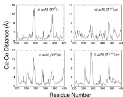
Fig. 3 C \alpha -C \alpha distances between two extreme protein structures projected from the 1st eigenvector obtained from essential dynamics analyses were performed for four models
