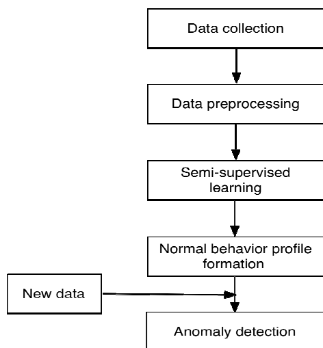
Fig. 1 Structure and major components of the semi-supervised network intrusion detection framework
