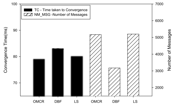
Fig. 6. Single Link Failure
