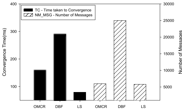
Fig. 8. Single Node Failure
