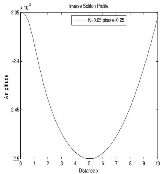
Fig. 3. Plot of Soliton Profile for Fixed Delta Varying K
