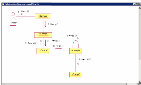
Fig. 5 Collaboration diagram
