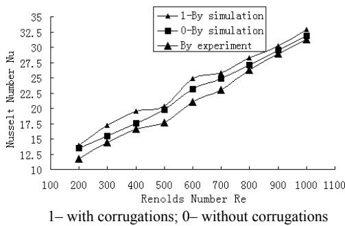
Fig. 11 Comparison of Nu in numerical simulation with experimental results
