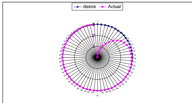
Fig. 4 Step Response of Proportional Controller
