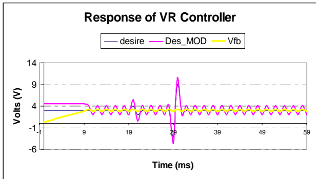
Fig. 10 Response of the VR Controller
