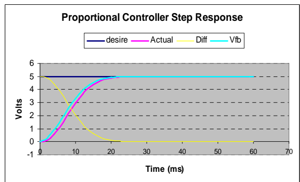
Fig. 5 Step Response of Proportional Controller
