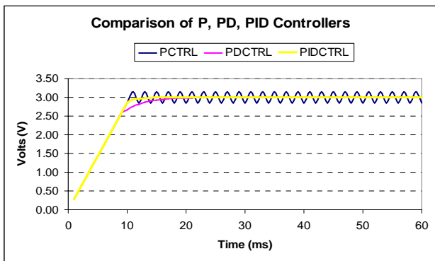
Fig. 6 Step Response of P, PD and PID
