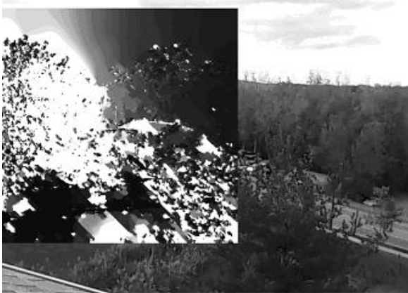
Fig. 2 Overlay of depth map in field of view of 2D frames, in the region of interest where target is tracked. White pixels appear as near to the camera, whereas black pixels appear as a far distance. The foliage is highlighted in part due to the non-simultaneous acquisition of the left and right stereo pairs from the webcam, in between which the foliage blows in the wind. Using a larger stereo baseline and post processing techniques would improve the quality of the depth map and hybrid algorithm performance
