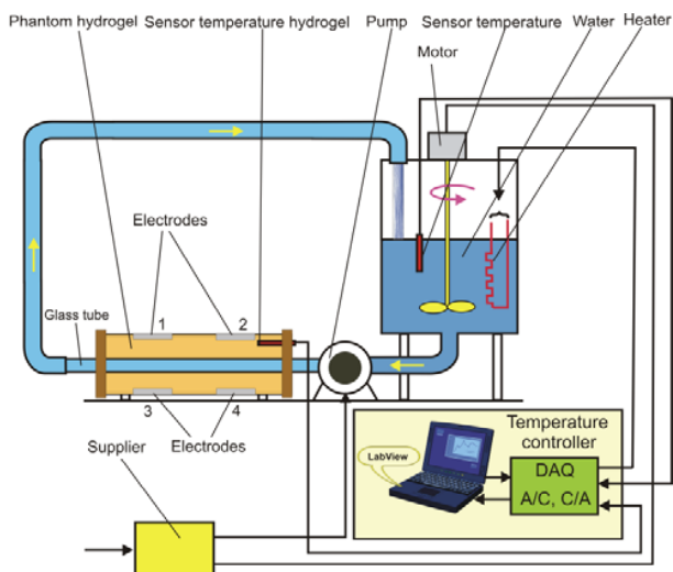
Fig. 13 The simplification of forearm's phantom scheme [12]
