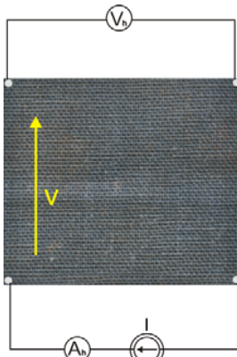
Fig. 2 Electric scheme for vertical resistance measurement [11]
