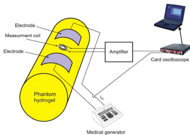
Fig. 14 The scheme of current measurement system under electrodes
