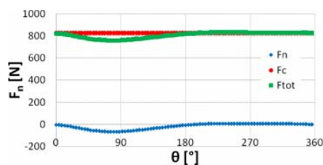
Fig. 13. Normal force F_n , centrifugal force F_c and total radial resultant force F_{tot} for \lambda = 3.09 .
