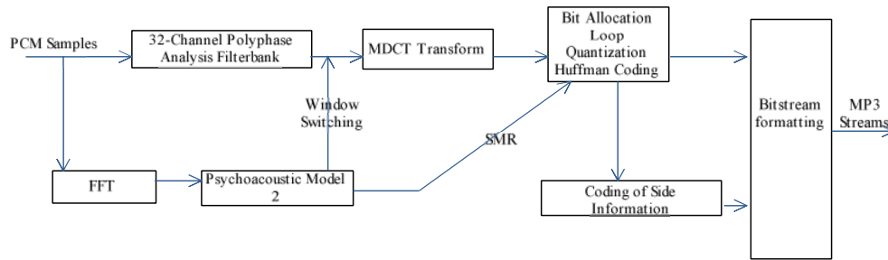
Fig.3.The flowchart of MP3 encoding
