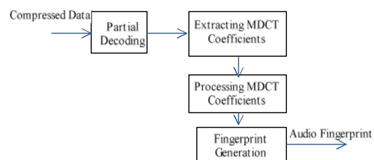
Fig.2. Block diagram of audio fingerprinting in compressed domain
