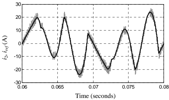
Fig. 8 Waveforms of current to be compensated (in black) and current i_2 (in gray) for L_2= 4\text{mH} and C_f=0.6\mu\text{F}
