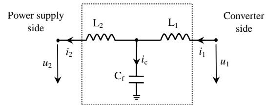
Fig. 2 Equivalent single phase diagram of the idealized LCL filter
