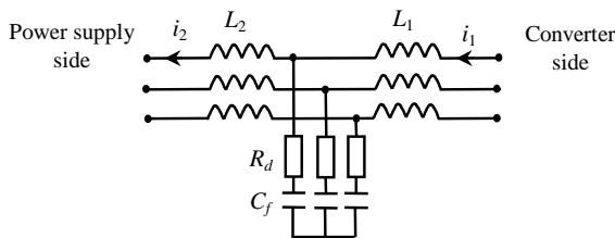
Fig. 12 LCL interface filter with damping resistors
