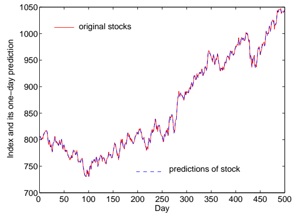
Fig. 3. The comparison of Dow 10 indexes and their one-day predictions through the MFP for 500 days from 2005-6-2 to 2007-5-31.
