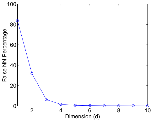
Fig. 2. The FNN plot of Dow 10 indexes for 2252 daily stock data from 1999/12/31 to 2007/12/10.
