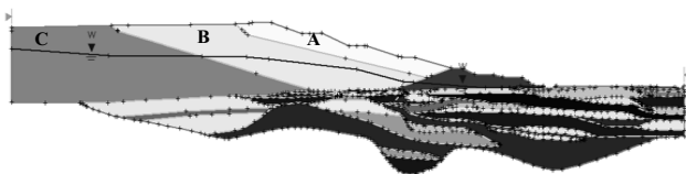
Fig. 2 The geological profile of cross-section no. 19
