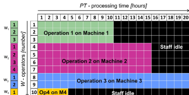
Fig. 1 Gantt type chart of investigated open shop staffing problem
