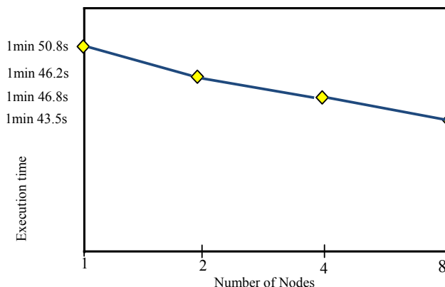
Fig. 4 Calculation Results on 1M Problem Size
