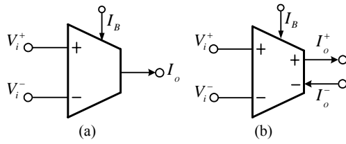
Fig. 1 The symbol of (a) the single ended OTA and (b) the fully differential OTA
