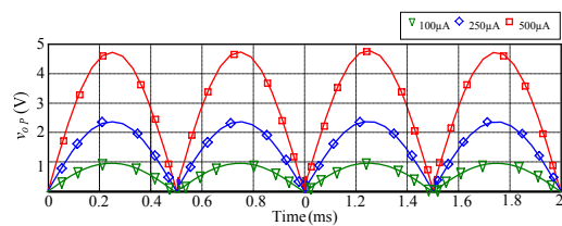
(a) positive full-wave rectifier
