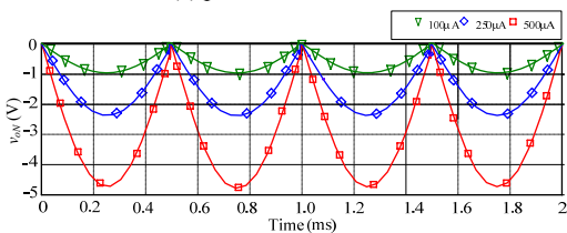
(b) negative full-wave rectifier
