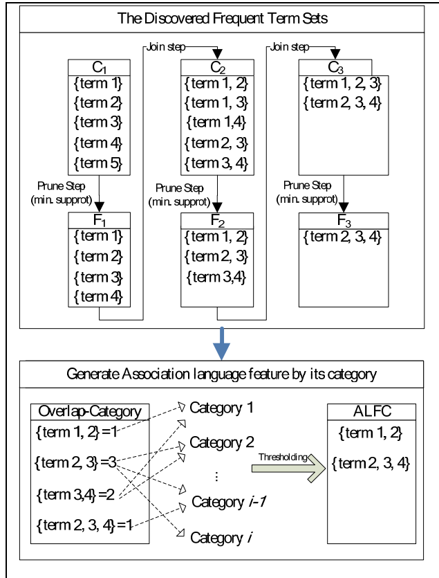
Fig. 1 Discover frequent term sets and generate association feature by its category
