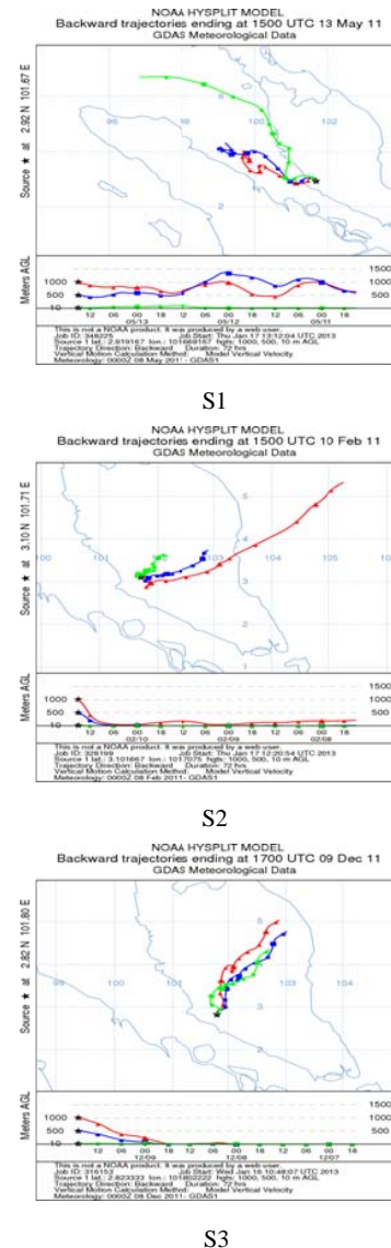
Fig. 4 Backward trajectory of wind direction for the Putrajaya (S1), Petaling Jaya (S2) and Nilai (S3) monitoring stations for the highest O_3 episode in 2011
