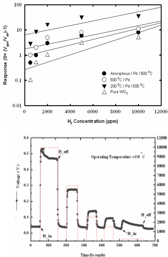
Fig.5 Response of pure and catalyzed films to different Hydrogen concentrations for samples at 350 °C (a) and a typical variation in electrical conductivity versus time for annealed film at 200 °C (b)
