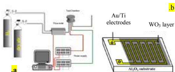
Fig.1 Schematic of gas sensing set up (a) and a typical sensor (b)
