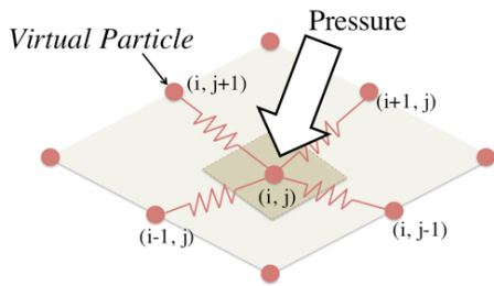
Fig. 7 Particle-based flexible membrane model
