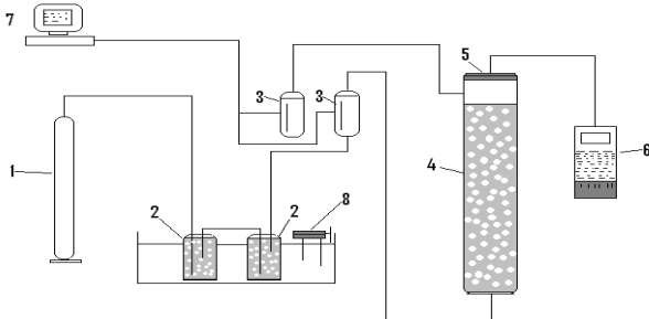
Fig. 1 Schematic diagram for experimental set-up
