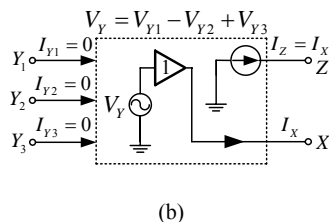
Fig. 1 DDCC (a) Symbol (b) Equivalent circuit
