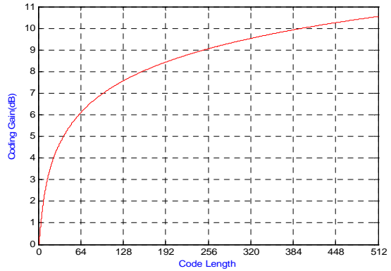
Fig. 1 SNR gain in the code-decode process
