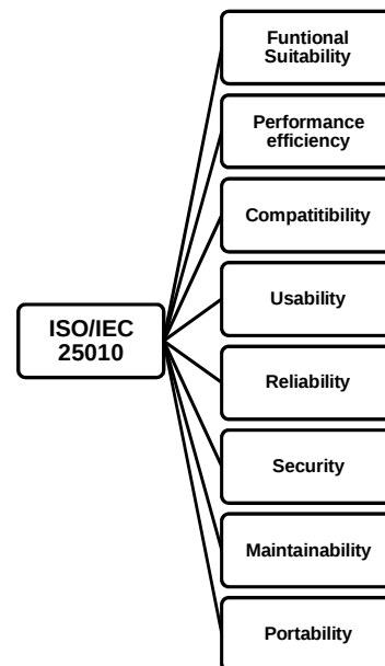
Fig. 2 ISO/IEC 25010 characteristics
