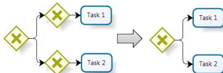
Fig. 4 Refactoring Operator 2
