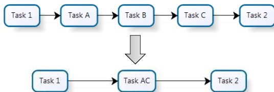
Fig. 11 Refactoring Operator 9
