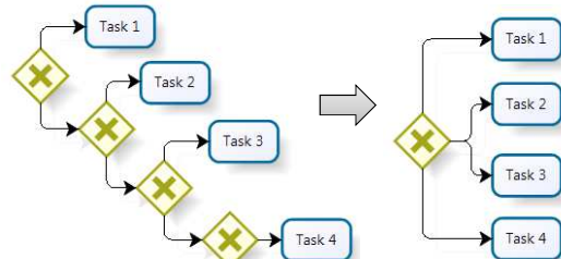
Fig. 5 Refactoring Operator 3
