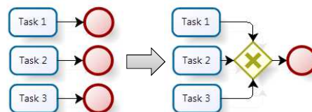
Fig. 10 Refactoring Operator 8
