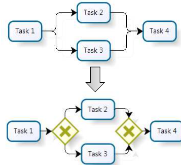
Fig. 8 Refactoring Operator 6
