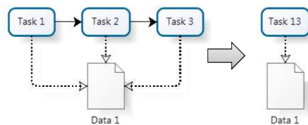
Fig. 7 Refactoring Operator 5
