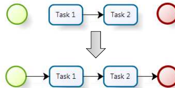
Fig. 9 Refactoring Operator 7
