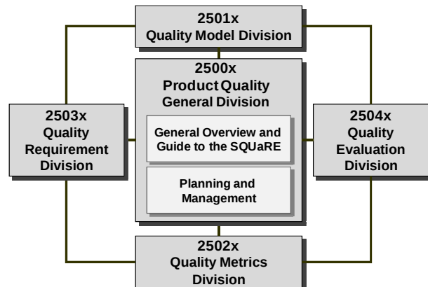
Fig. 1 ISO/IEC 25000 divisions.
