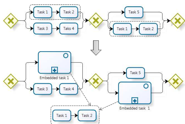
Fig. 6 Refactoring Operator 4
