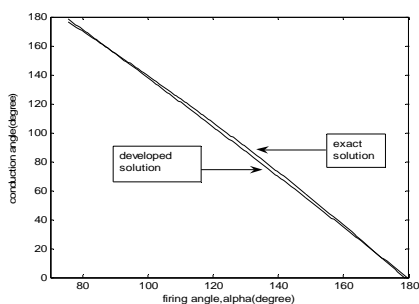
Fig. 6 Variation of firing angle ( \alpha ) with conduction angle ( \delta ) in case of \theta = 75^\circ
