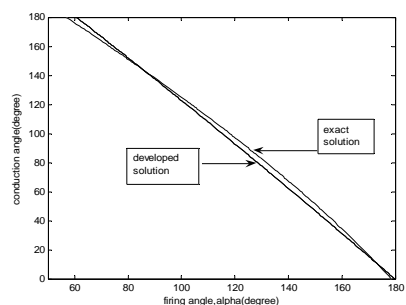
Fig. 5 Variation of firing angle ( \alpha ) with conduction angle ( \delta ) in case of \theta = 55^\circ
