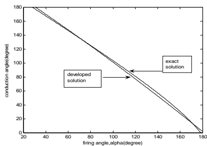
Fig. 4 Variation of firing angle ( \alpha ) with conduction angle ( \delta ) in case of \theta = 25^\circ
