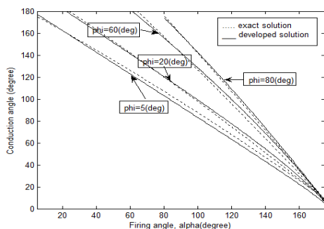
Fig. 7 Variation of firing angle ( \alpha ) with conduction angle ( \delta ) for difference cases of load angle ( \theta )
