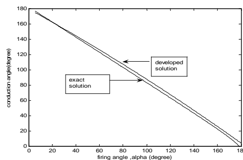
Fig. 3 Variation of firing angle ( \alpha ) with conduction angle ( \delta ) in case of \phi = 5^\circ
