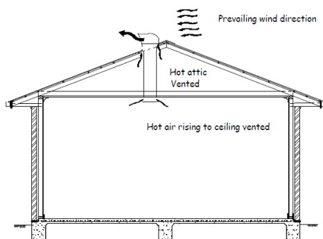
Fig. 4 Wind directional skylight vent on house roof
