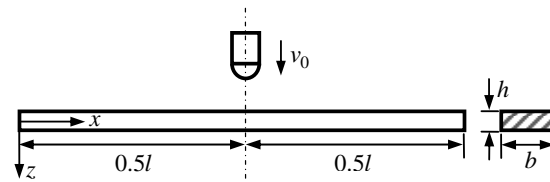
Fig. 1 Structure model
