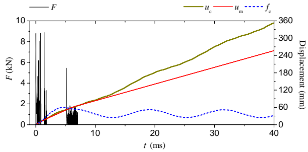
Fig. 4 Response of impact force and displacement
