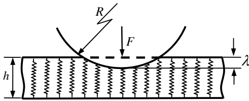
Fig. 2 Uniaxial compression elastic-plastic contact model
