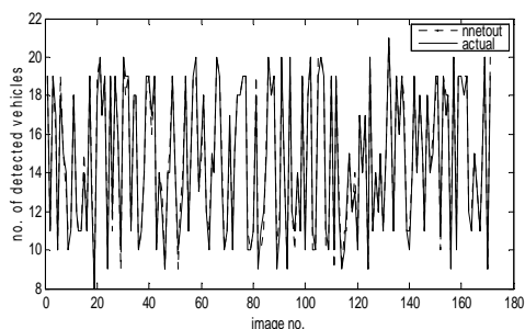
Fig. 8 Actual and neural network outputs
