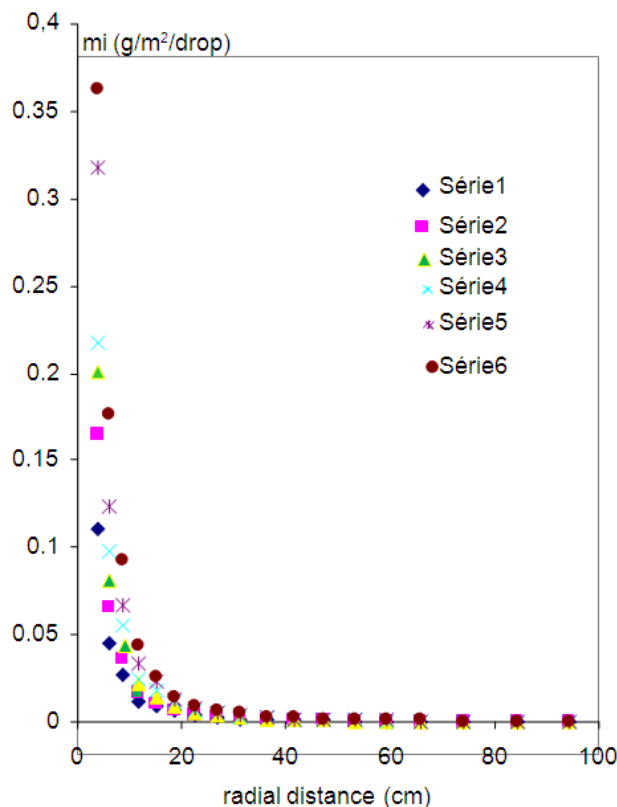
Fig. 6 The relationship between the splashed mass m_i (g/m²/drop) in the compartments and the radial distance for different slope angles. [serie1: 0°, serie2: 2°, serie3: 5°, serie4: 10°, serie5: 17° and serie6: 20°]
