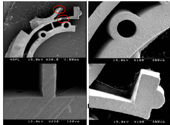
Fig. 6 sintered samples
