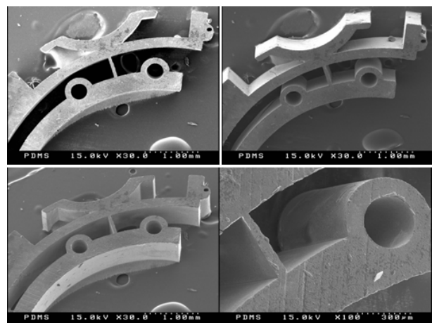
Fig. 4 Green Samples
