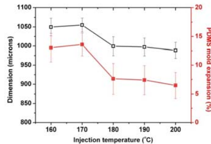
Fig. 3 Effect Injection temperature on green part dimension
