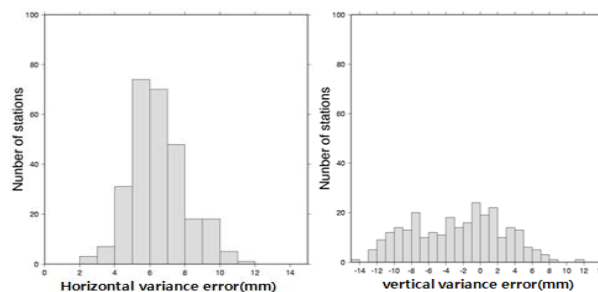
Fig. 4 Horizontal and vertical distribution of the differences (mm)
