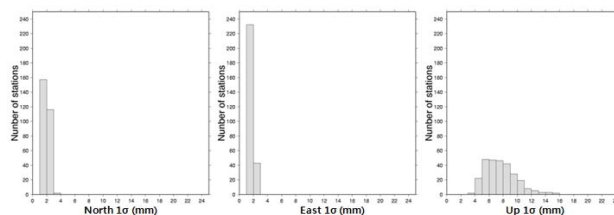
Fig. 3 Distribution of accuracy level of each constituent
