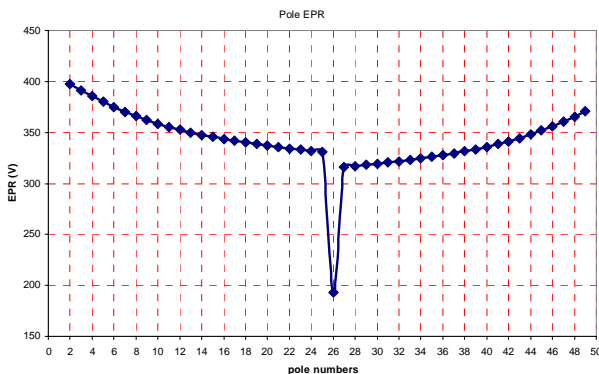
Fig. 12 Pole fault along the transmission line
