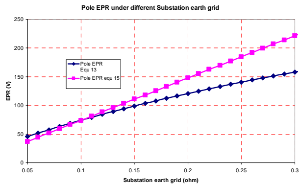
Fig. 10 Pole EPR under different substation earth grid
