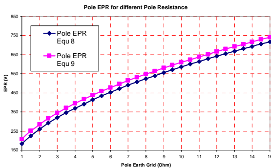
Fig. 4 EPR for pole fault with equations 8 and 9
