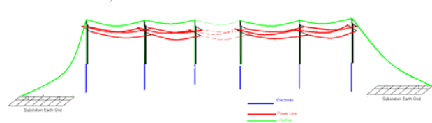
Fig. 1 OH transmission mains layout with OHEW
