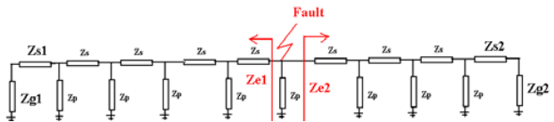
Fig. 8 Pole fault for finite transmission line
