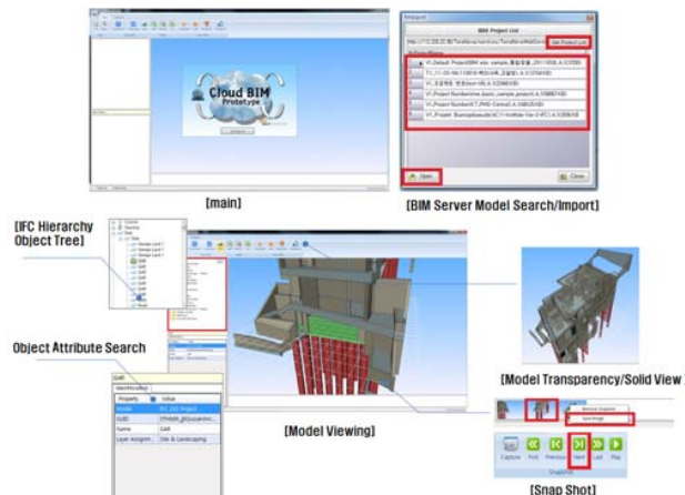
Fig. 7 Main Screen by Functions of the BIM Server Based Viewer
