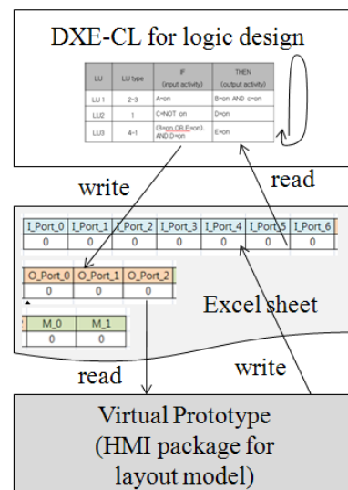
Fig. 9. Structure of virtual prototype
